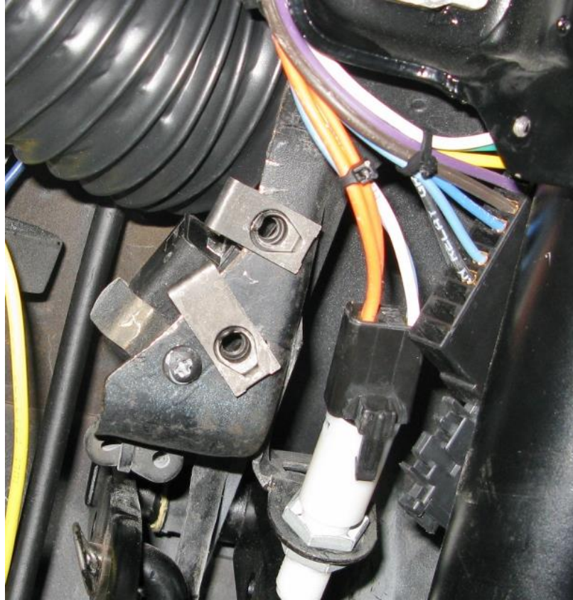
Figure 13 - Install U-nuts
